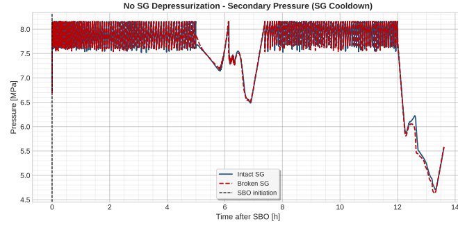
Figure 14: Secondary Pressure.
